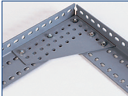
Connector Plate
