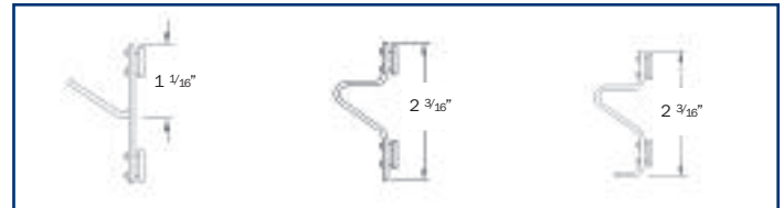
Heavy Angle Post T-Post Heavy T-Post
